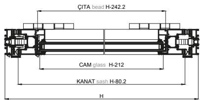
1 KESİTİ section 1
