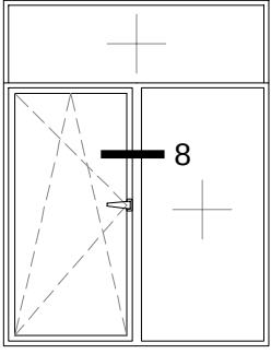
BİNİLİ İÇE AÇILIR ORTA KAYITLI DETAY OVERLAPPING INWARD OPENING DETAIL WITH MULLION
