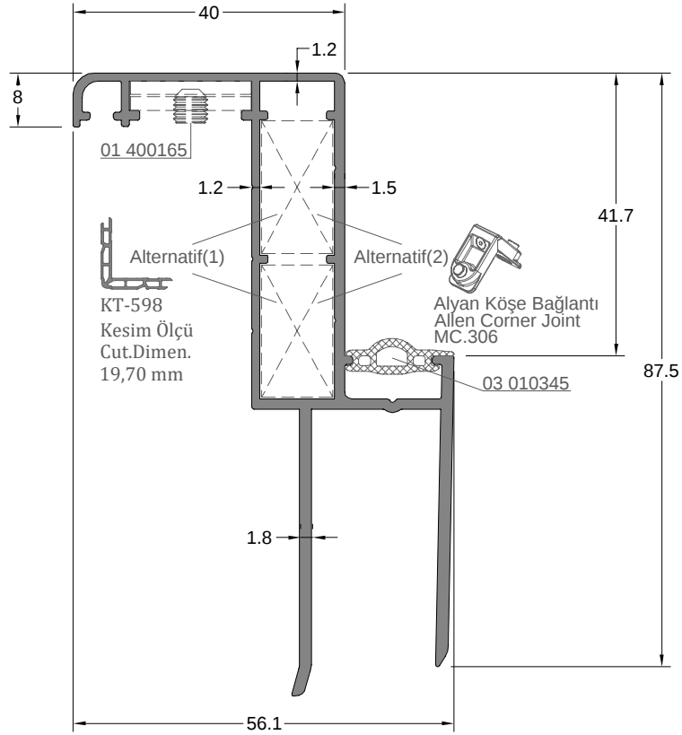
Kasa Profili FRAME PROFILE
