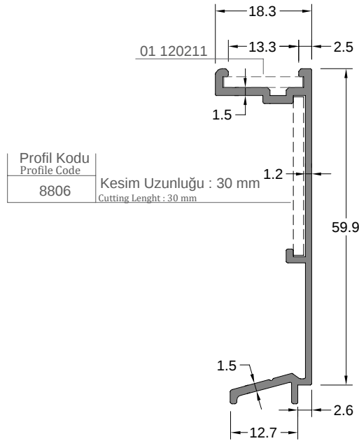
Pervaz Eki Profili SILL JOINT PROFILE
