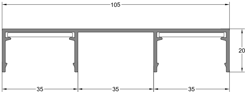
Yan Kapak Profili SIDE COVER PROFILE
