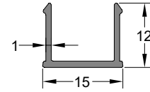
Kapak Profili COVER PROFILE
