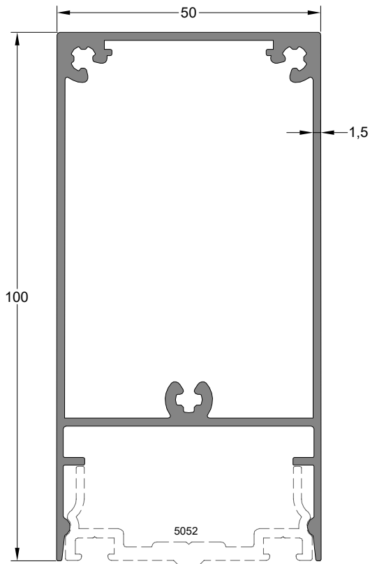
Badem Kapak Profili ALMOND COVER PROFILE
