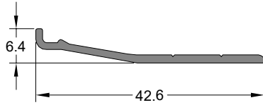
Tek Cam ve Spandrel Panel Kaset Profili SINGLE GLAZING AND SPANDREL PANEL CASSETTE PROFILE
