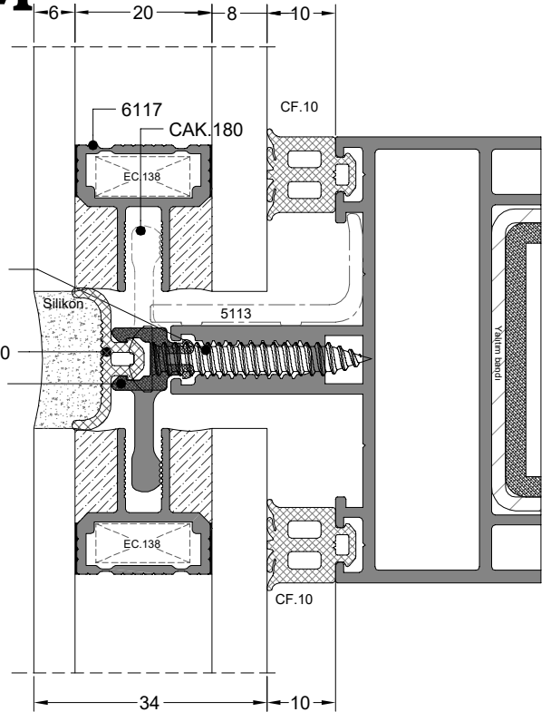
YATAY DETAYI HORIZONTAL DETAIL
