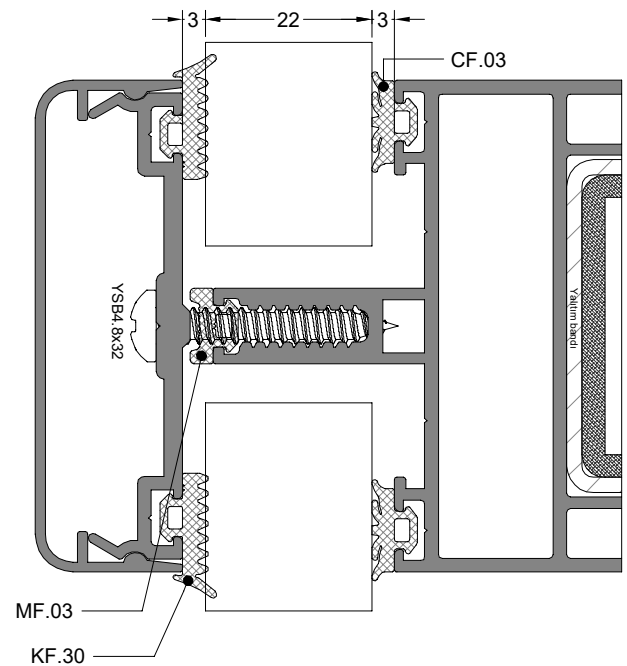
YATAY DETAYI HORIZONTAL DETAIL
