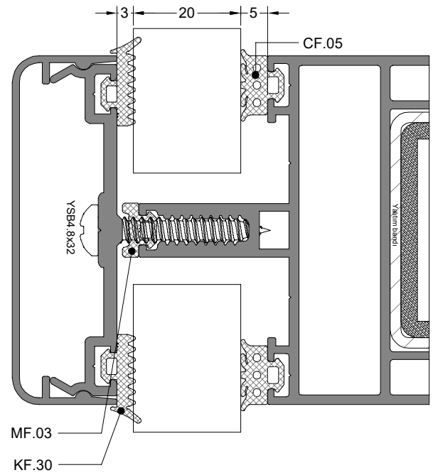
YATAY DETAYI HORIZONTAL DETAIL
