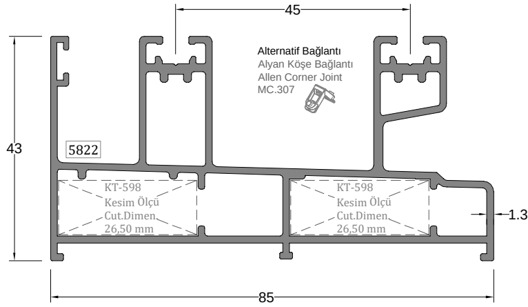
İki Raylı Kasa Profili DOUBLE RAIL FRAME PROFILE
