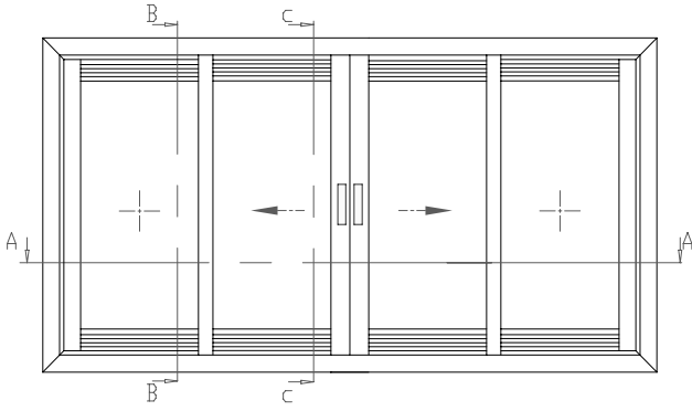
PROFİLLER / PROFILES
