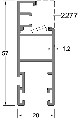
Sineklik Profili SCREENING PROFILE
