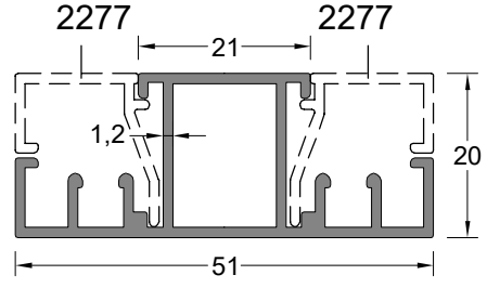
Sineklik Profili SCREENING PROFILE
