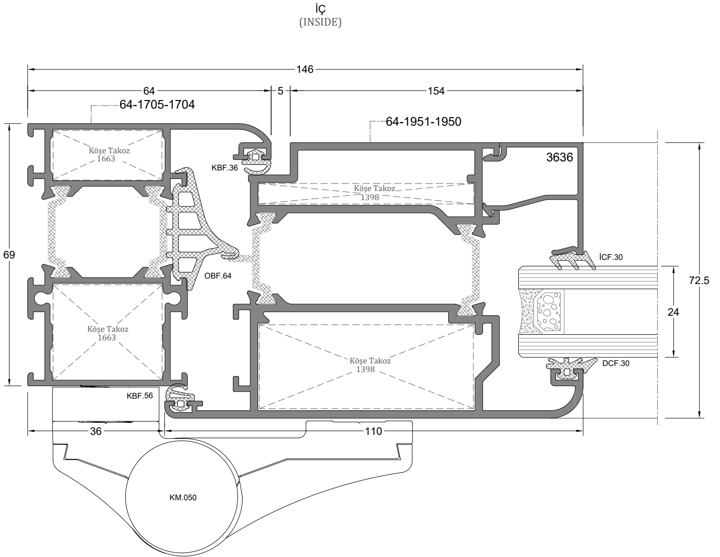
DİŞA AÇILIR BİNİLİ KAPI DETAY OUTWARD OPENING OVERLAPPING DOOR DETAIL
